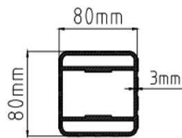
Tennis post Sectional Drawing
